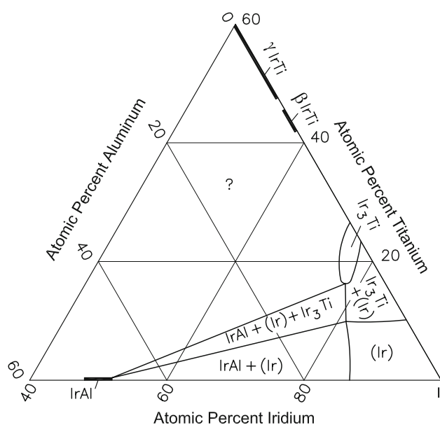
Fig. 2 Al-Ir-Ti partial isothermal section at 1650 °C for Ir-rich alloys [2005Miu]
