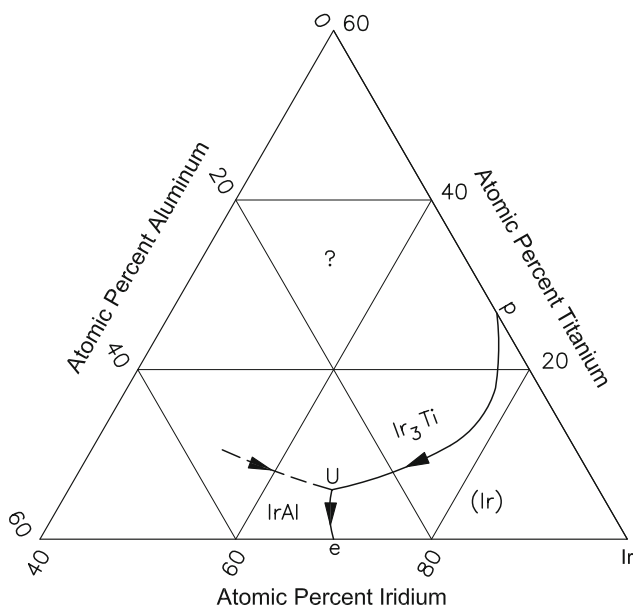
Fig. 1 Al-Ir-Ti partial liquidus projection for Ir-rich alloys [2005Miu]
